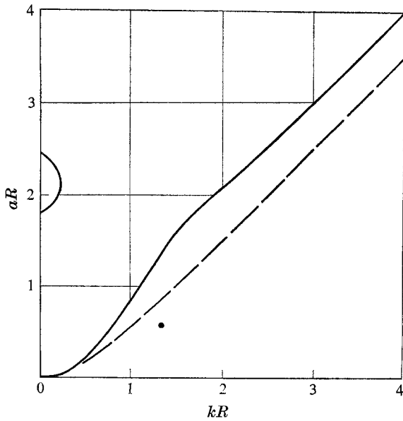
FIGURE 31. Spatial amplification rate as a function of wave-number. The solid curves result from the theory of spatially growing waves, and the dashed curve results from a transformation of temporal theory. The experimental datum is the maximum amplification rate of the preferred fundamental, as determined from figure 24.
