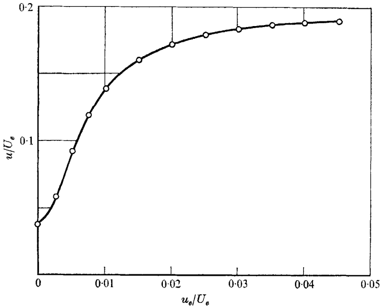
FIGURE 10. Amplitude response at the preferred Strouhal number 0.30. The response u/U_e is measured on the centreline four diameters downstream of the jet exit.
