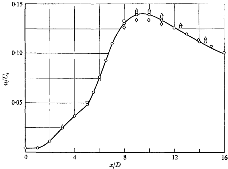
FIGURE 8. Profile of the root-mean-square axial fluctuation on the centreline. The data symbols are defined in the caption of figure 7.
