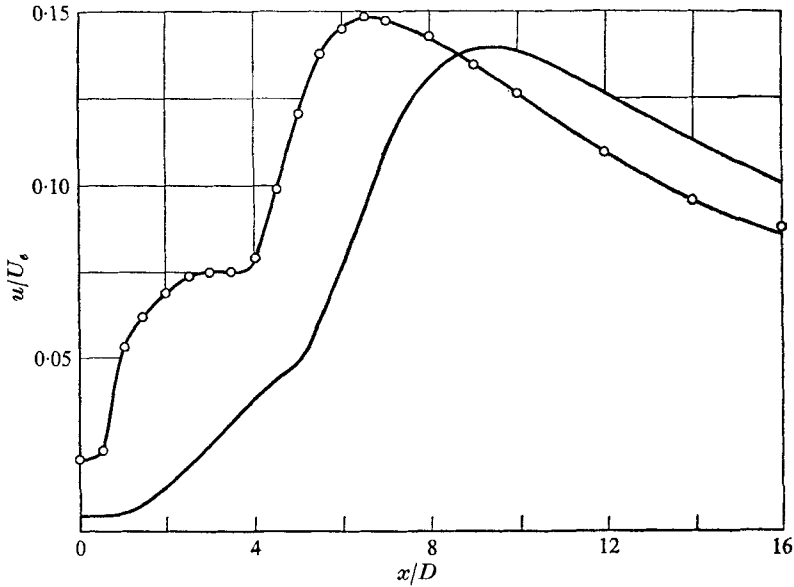
FIGURE 22. Centreline profile of turbulence intensity under 2% forcing at a Strouhal number of 0.60. The curve without data points represents the unforced case and is taken from figure 8.
