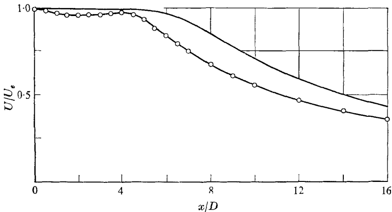
FIGURE 23. Mean-speed decay along the centreline under 2% forcing at a Strouhal number of 0.60. The curve without data points is the unforced profile taken from figure 7.
