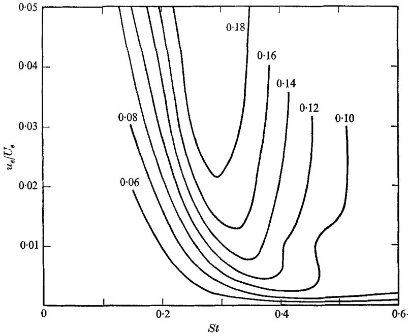
FIGURE 18. Contour map of the total response four diameters downstream on the centre-line, as a function of Strouhal number and amplitude of forcing. The contours are labelled with u/U_e , which rises by 0.02 from one curve to the next. The abscissa is the contour u/U_e = 0.04 approximately, the turbulence intensity in the absence of forcing.
