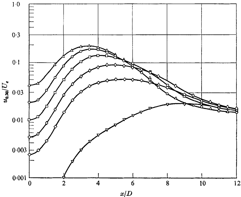
FIGURE 24. Centreline intensity profiles of the fundamental wave driven at a Strouhal number of 0.30. The data symbols denote the following forcing amplitudes u_e/U_e : \nabla , no forcing; \diamond , 0.25%; \diamond , 0.5%; \square , 1%; \circ , 2%; \triangle , 4%. The ordinate u_{0.30}/U_e is logarithmic, so the forced profiles would have had the same shape had the jet been linear.
