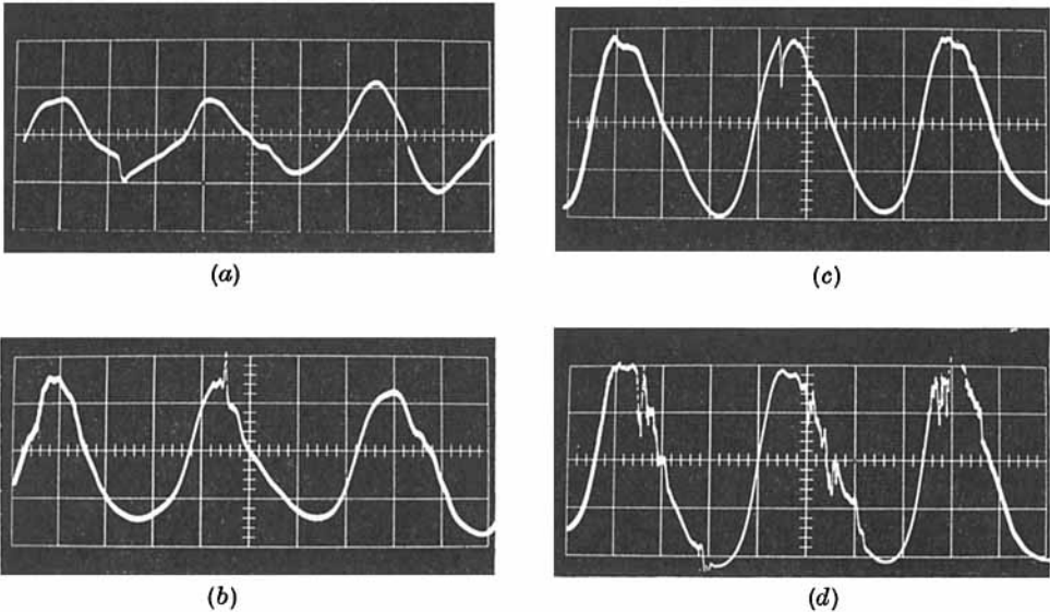
FIGURE 11. Wave-forms of the preferred mode, measured on the centreline four diameters downstream of the exit. The Strouhal number is 0.30 and the forcing amplitudes u_e/U_e are (a) 0.5%, (b) 1%, (c) 2%, and (d) 4%.
