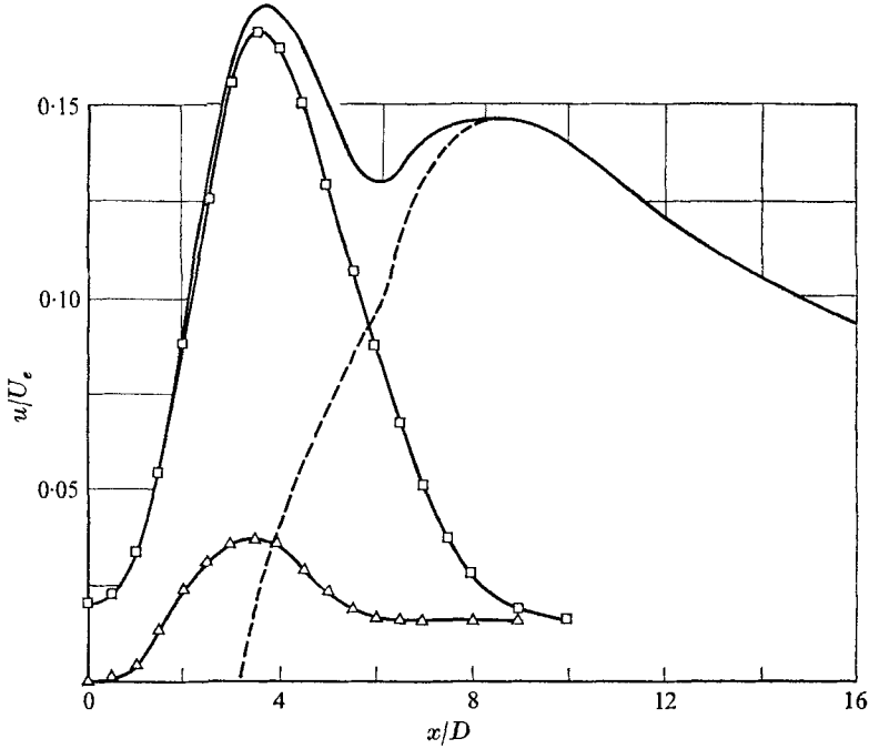
FIGURE 14. Filtered axial profiles of the preferred mode. The solid curve without data points represents the total intensity u/U_e and is taken from figure 13. The square data symbols denote the contribution u_{0.30}/U_e of the fundamental, and the triangular symbols denote the contribution u_{0.60}/U_e of the harmonic. The dashed curve represents the intensity of turbulence not bound in the fundamental or harmonic.
