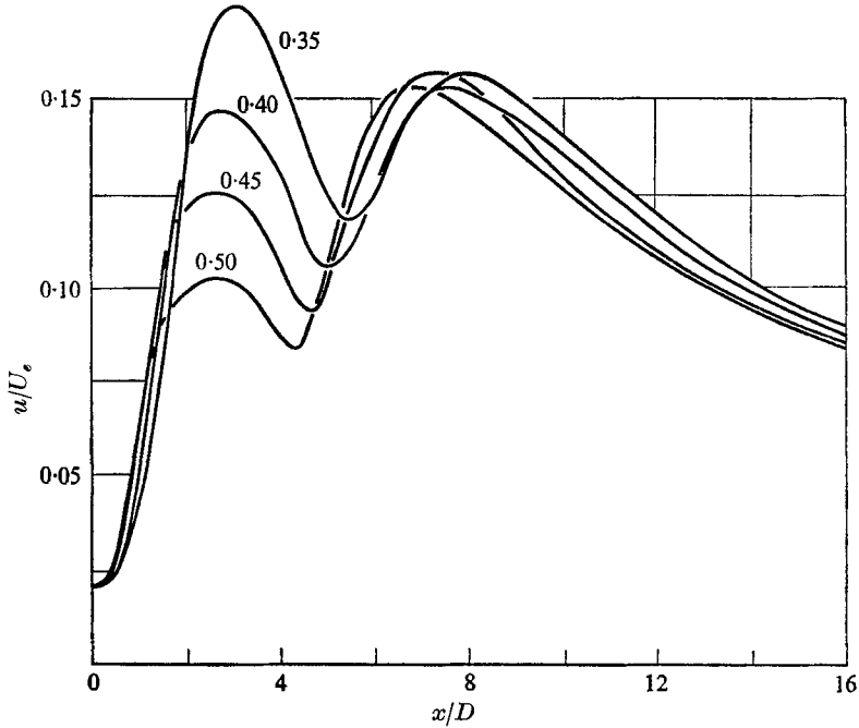
FIGURE 20. Centreline profiles continued through the Strouhal-number interval 0.35 to 0.50.
