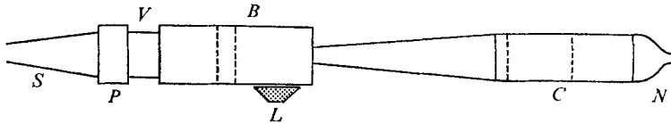
FIGURE 3. Schematic of the jet facility, which is about 16 ft long. The dotted lines represent grids or screens, and the labelled parts are described in the text.
