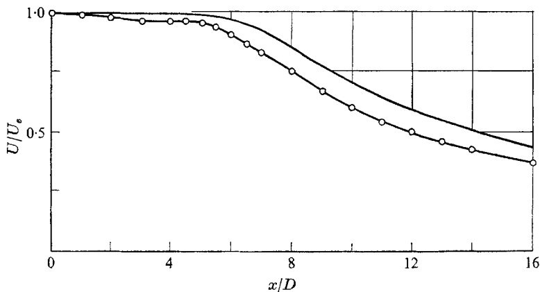
FIGURE 15. Effect of the preferred mode on the decay of mean speed along the centreline. The forcing level is 2%, and the Strouhal number is 0.30. The profile without data points represents the unforced case and is based on figure 7.
