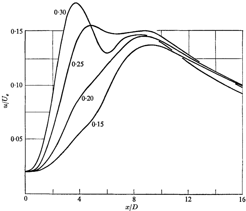
FIGURE 19. Centreline profiles of turbulence intensity, under 2% forcing in the Strouhal-number interval 0.15 to 0.30. The Strouhal numbers are given on the plot.
