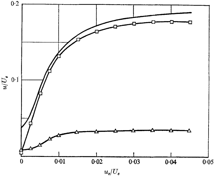
FIGURE 12. Filtered response functions of the preferred mode. The experimental conditions are the same as for figure 10, from which the curve without data points is taken, representing the total intensity u/U_e . The square data symbols denote the fundamental response u_{0.30}/U_e , and the triangular symbols denote the harmonic response u_{0.60}/U_e .
