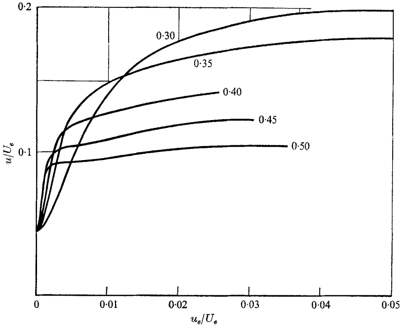
FIGURE 17. Amplitude-response functions continued through the Strouhal-number interval 0.30 to 0.50.
