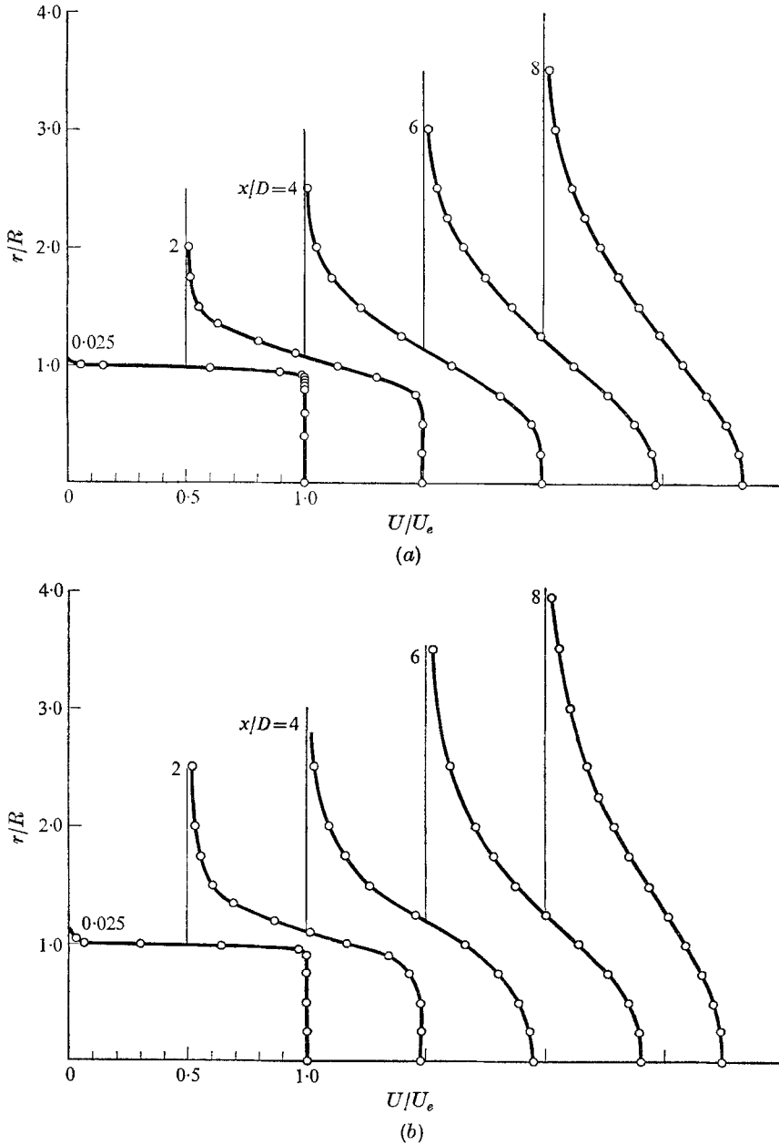
FIGURE 27. Radial mean-speed profiles at five stations along the jet axis: (a) without forcing, and (b) with 2% forcing at a Strouhal number of 0.30. The stations x/D are specified near the ordinates of the profiles, which are arranged to suggest the spatial structure of the jet.
