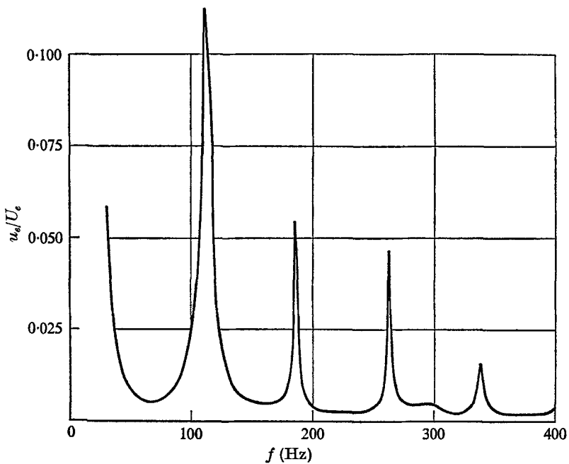
FIGURE 9. Spectrum of the jet cavity, measured in terms of the root-mean-square surging in the exit plane.
