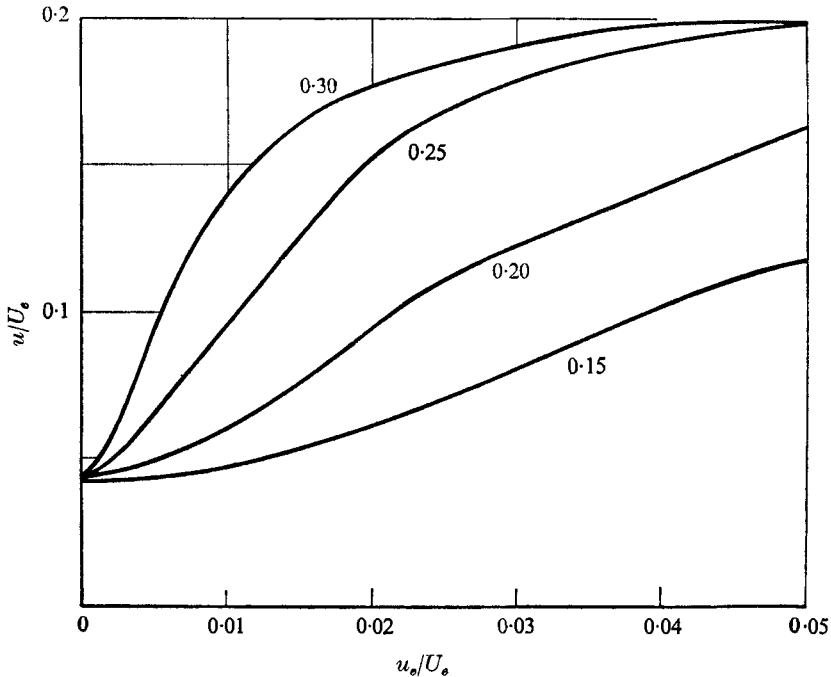
FIGURE 16. Amplitude-response functions measured on the centreline four diameters downstream of the jet exit. The response functions are labelled with Strouhal numbers, which range from 0.15 to 0.30.
