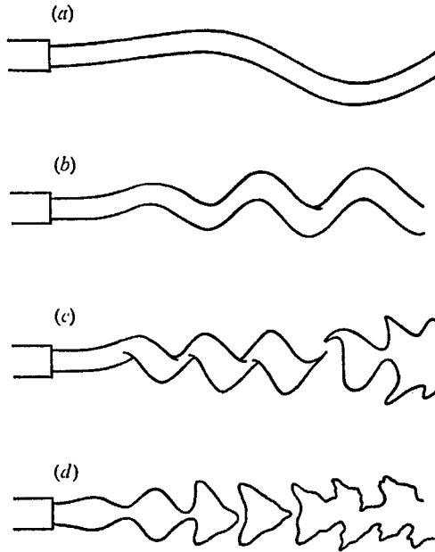
FIGURE 2. Evolution of jet instability with advancing Reynolds number. Parts (a)–(d) span the Reynolds-number interval from around 10^2 to 10^3 .
