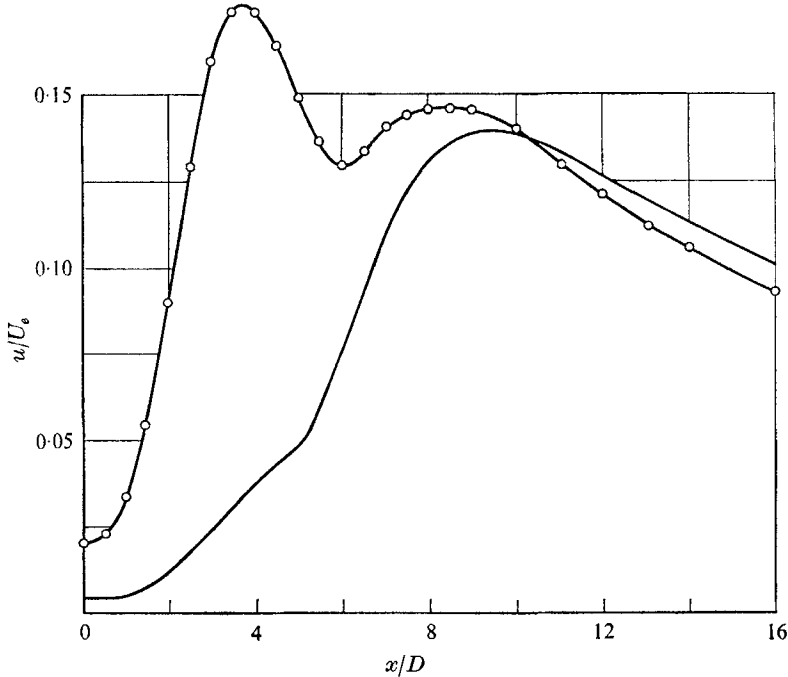
FIGURE 13. Axial profile of the turbulence intensity, measured along the centreline under 2% forcing at a Strouhal number of 0.30. The curve without data points represents the unforced case and is taken from figure 8.
