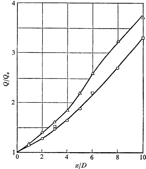
FIGURE 29. Axial profiles of volume flux, normalized on the flux out the jet exit. The round data symbols denote the unforced case, and the square symbols represent comparable data from Sami et al. (1967). The triangular symbols denote the case of 2% forcing at a Strouhal number of 0.30.
