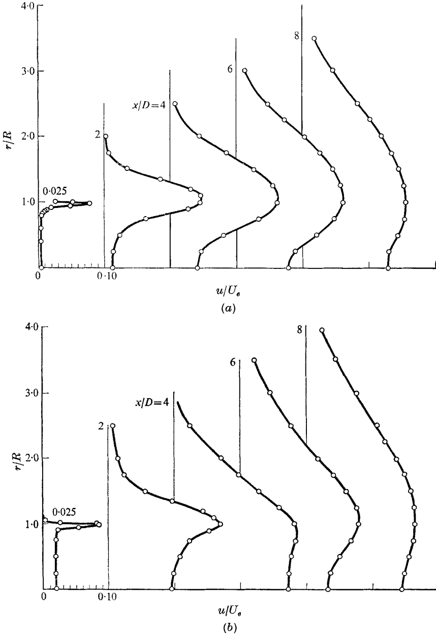
FIGURE 28. Radial intensity profiles of the axial component of turbulent velocity: (a) unforced, and (b) forced at a level of 2% and a Strouhal number of 0.30.
