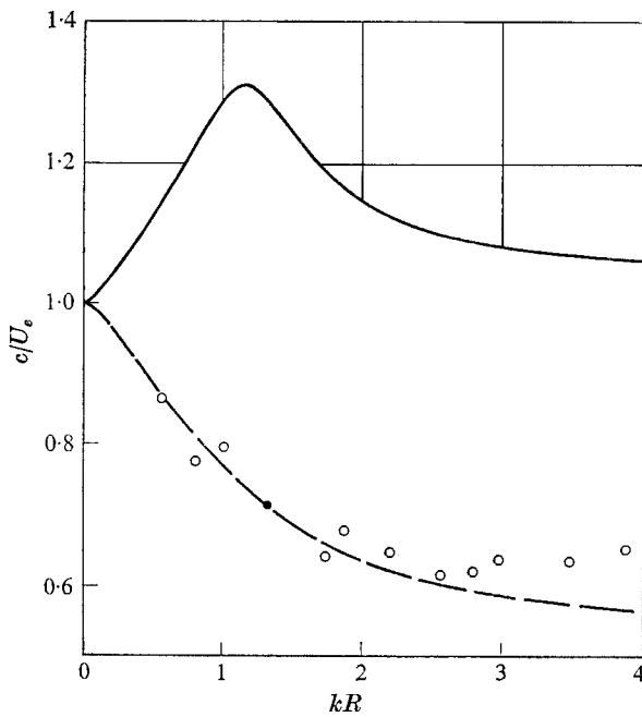
FIGURE 32. Phase velocity as a function of wave-number. The solid curve represents spatial theory and the dashed curve temporal. The data are computed from table 4.
