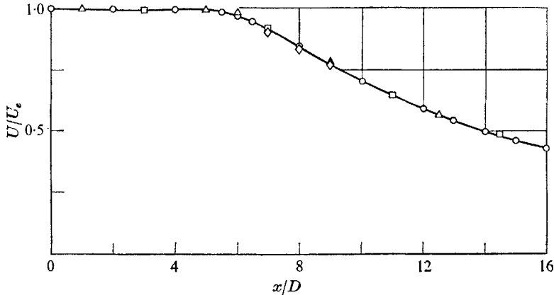
FIGURE 7. Profile of the mean axial speed on the centreline at several Reynolds numbers, as denoted by the following data symbols: \Delta , 6.2 \times 10^4 ; \square , 8.3 \times 10^4 ; \circ , 1.03 \times 10^5 ; and \diamond , 1.24 \times 10^5 .
